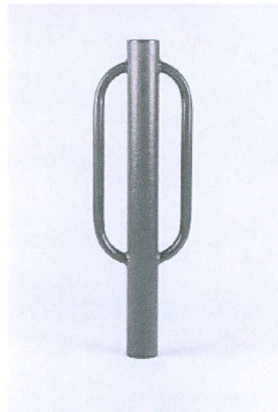
17A 28" Overall Length 2 3/8" ID 17B 28" Overall Length 3" ID 17C 28" Overall Length 3 1/2" ID
